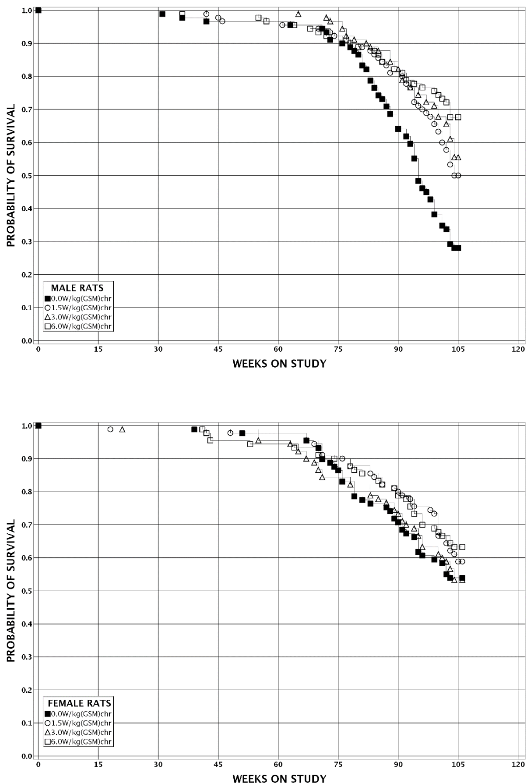
FIGURE 7 Kaplan-Meier Survival Curves for Rats Exposed to GSM-Modulated Cell Phone RFR for 2 Years
