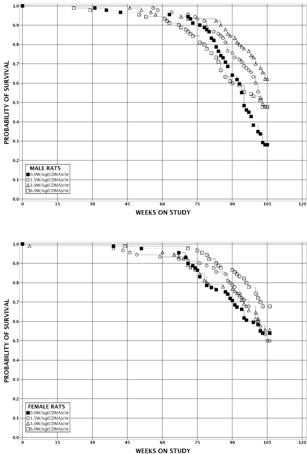
FIGURE 10 Kaplan-Meier Survival Curves for Rats Exposed to CDMA-Modulated Cell Phone RFR for 2 Years
